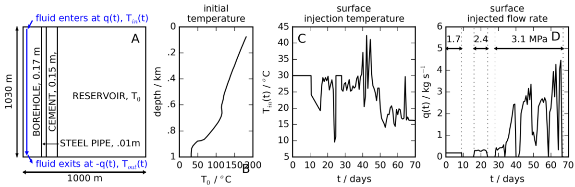
1058 Figure 3: Set up and inputs for the wellbore model. (A) Schematic showing modeled components (with 1059 widths) of the wellbore, as well as fluid entry and exit points. Material properties for the each of the zones 1060 are given in Table 1. The blue arrow shows the passage of the wellbore fluid. (B) Static down-hole 1061 temperature profile used as an initial temperature, T_0 , distribution for both the wellbore and stimulation 1062 models. (C) Surface injection temperature, T_{in}(t) , and (D) injection rate, q(t) , with time. These are 1063 applied as fluid entry boundary conditions in (A). Duration of the three pressure stimulations are indicated 1064 by dotted lines in (D).
