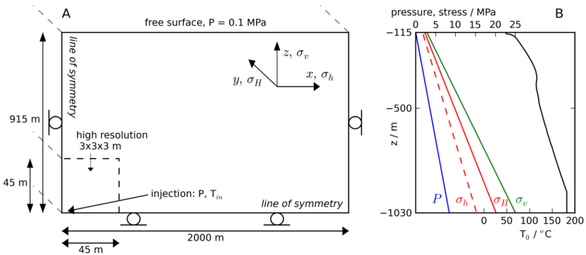
Figure 6: Set up and initial conditions for the stimulation model. (A) Schematic representation of the model grid in one eighth symmetry. Injection occurs into the bottom corner node contained within a high-resolution section of the grid. No flow and roller boundary condition are applied at all boundaries except the top surface, which is free to deform and fixed at atmospheric pressure. Orientation of the principal stresses relative to the coordinate axes is indicates in the top right. (B) Depth-dependent pressure, stress components and temperature applied as an initial condition. Initially, there is no horizontal variability in these variables.
