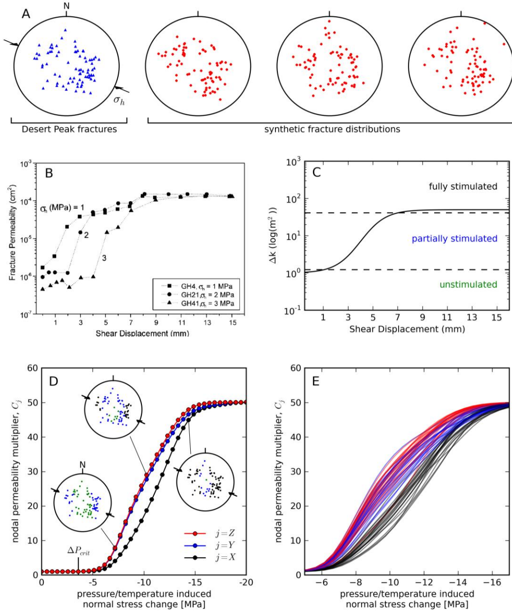
Figure 5: Summary of stress-permeability model (A). Equal-area stereonets showing poles to planes for the fracture population observed in image logs over the Desert Peak stimulation interval (blue triangles; [27]), and several synthetic fracture populations (red circles), generated from (A) using the algorithm described in Section 4.1. The orientation of \sigma_h is shown for the Desert Peak fractures. (B) Fracture permeability versus shear displacement for laboratory tests on granite at three normal stresses, from Lee and Cho [43]. (C) Modeled curve (Eq. (6)), with \Delta k_{max}=1.7 , u_5=1 mm and u_{95}=7 mm. Dashed lines divide regions defining fractures that are unstimulated ( \Delta k < 0.05\Delta k_{max} ), partially stimulated ( 0.05\Delta k_{max} < \Delta k < 0.95\Delta k_{max} ), and fully stimulated ( 0.95\Delta k_{max} < \Delta k ). Note that because \Delta k is used as a
